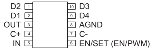
SC70JW-10 (Top View)
