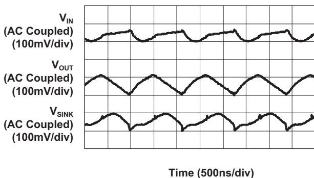
AAT3195-1 Output Ripple Waveform (V IN = 3.6V; 2X Mode; 30mA Load)
