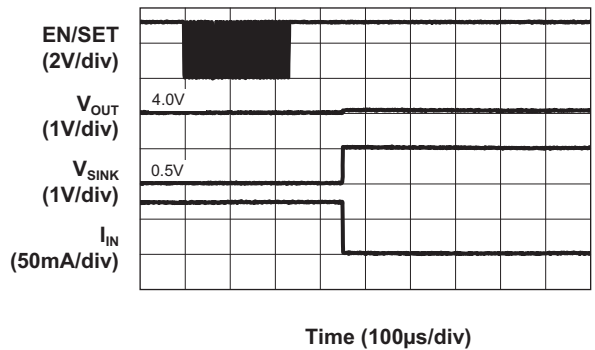
Transition of LED Current (20.5mA to 1.3mA)
