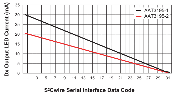
Figure 2: AAT3195-1/-2 Current Control Profile
