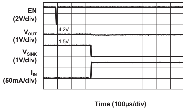
Transition of LED Current (1.3mA to 20.5mA)
