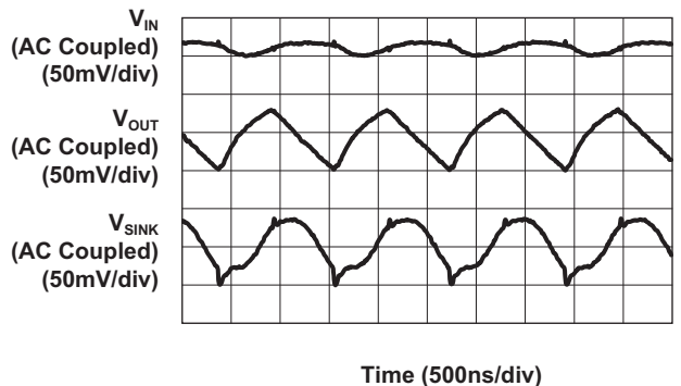
AAT3195-2 Output Ripple Waveform (V IN = 3.6V; 2X Mode; 20.5mA Load)
